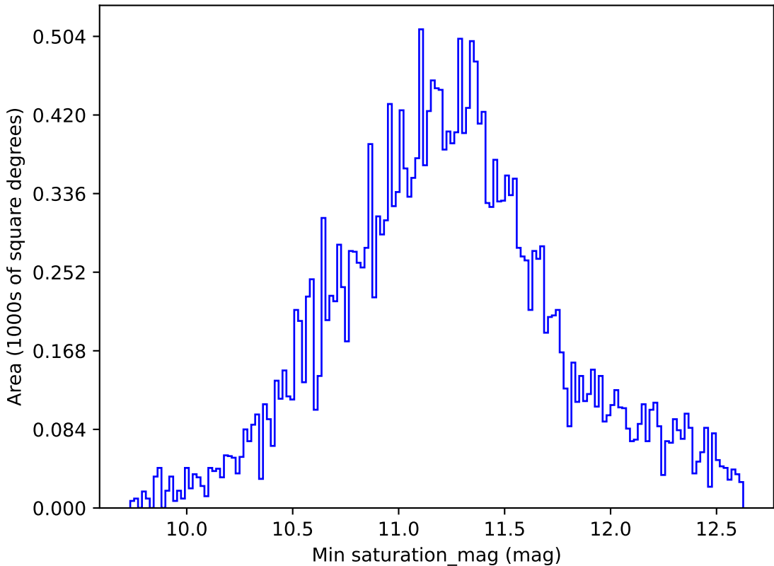
weather_cloudso2v3.4_10yrs All sky all bands: Min saturation_mag
