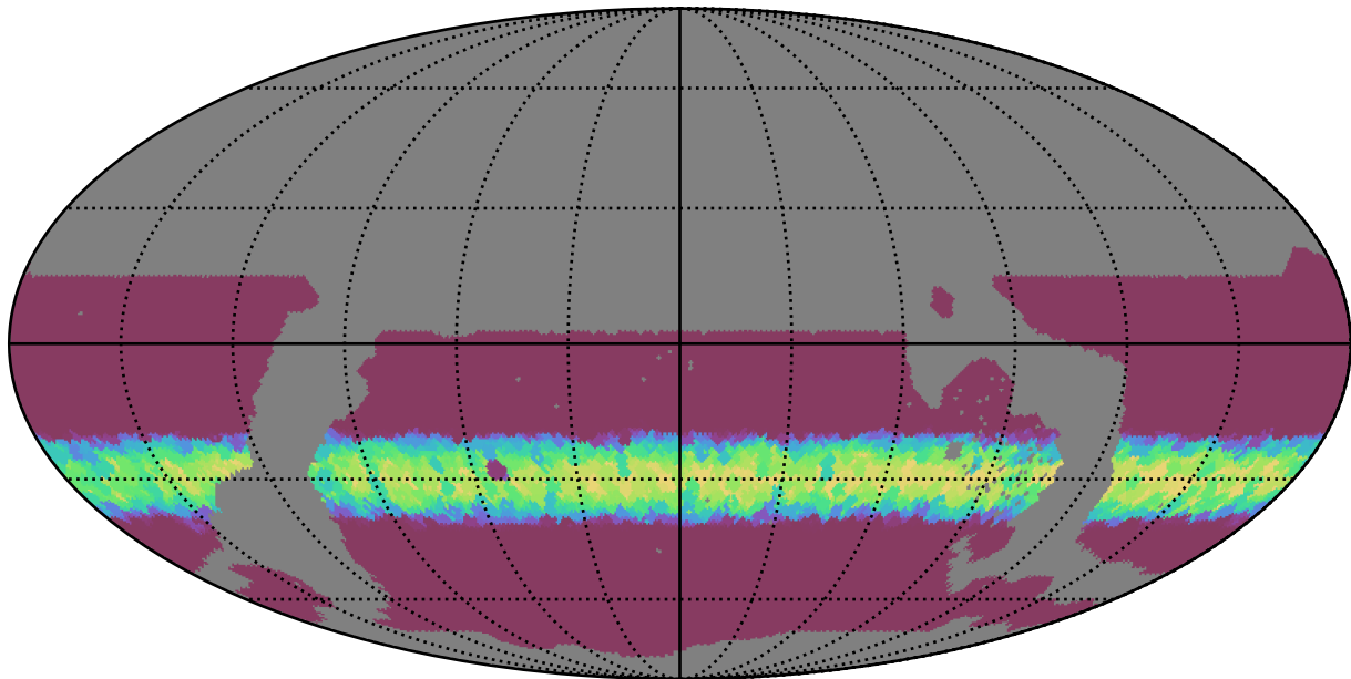
weather_cloudso2v3.4_10yrs WFD all bands: Min normairmass
