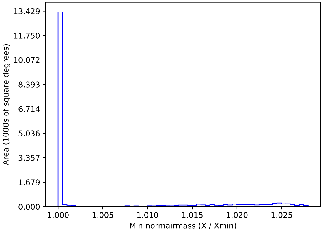
weather_cloudso2v3.4_10yrs WFD all bands: Min normairmass
