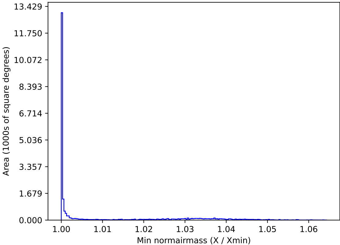
weather_cloudso2v3.4_10yrs All sky u band: Min normairmass
