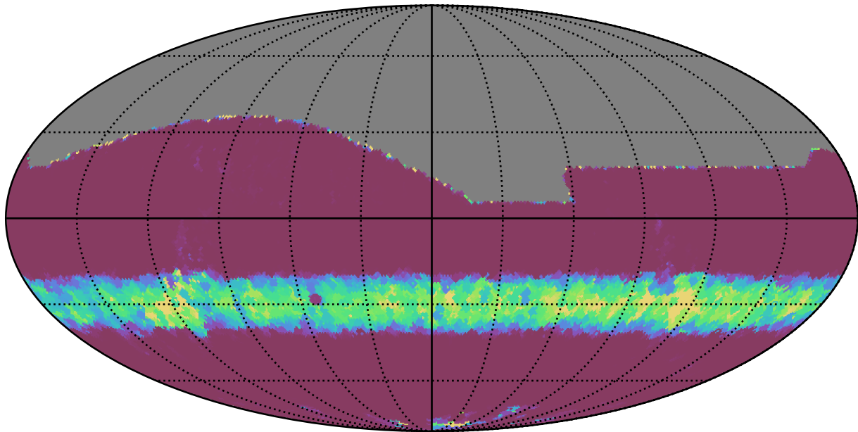
weather_cloudso2v3.4_10yrs All sky r band: Min normairmass
