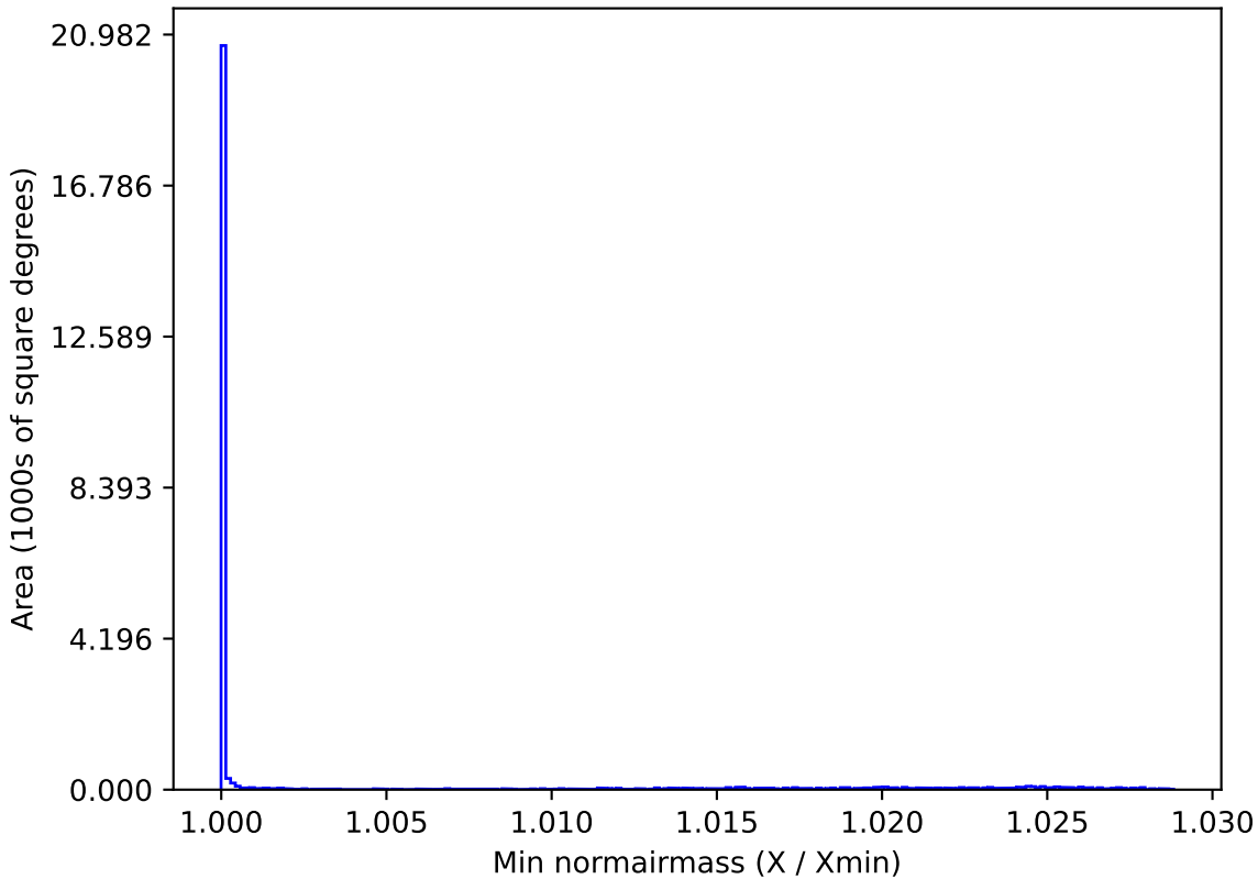
weather_cloudso2v3.4_10yrs All sky all bands: Min normairmass
