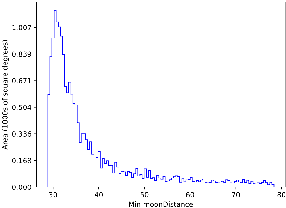
weather_cloudso2v3.4_10yrs WFD r band: Min moonDistance
