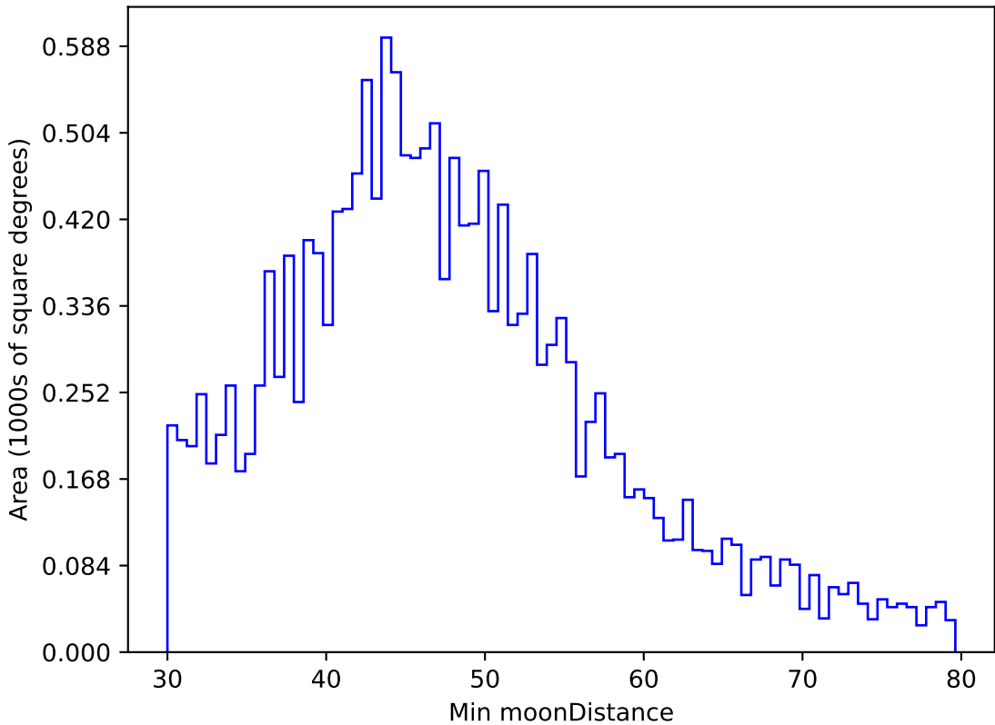
weather_cloudso2v3.4_10yrs WFD g band: Min moonDistance
