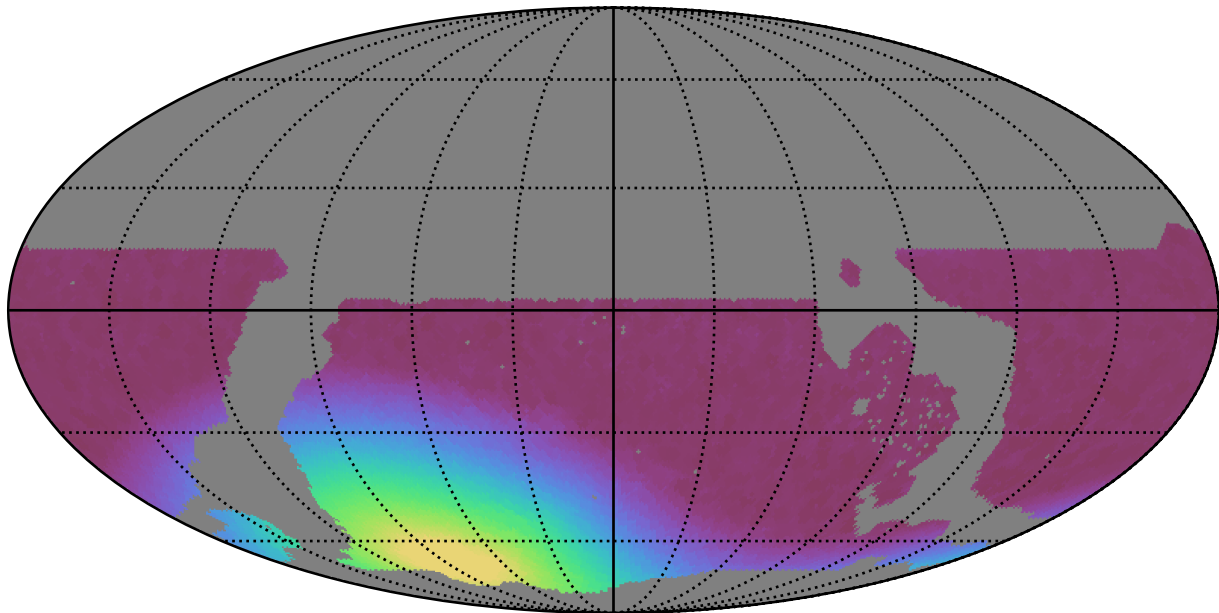
weather_cloudso2v3.4_10yrs WFD all bands: Min moonDistance
