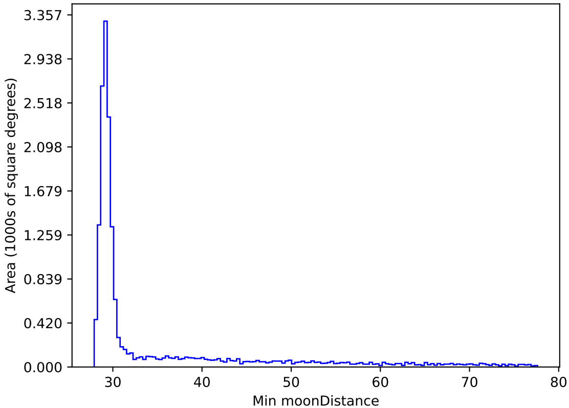
weather_cloudso2v3.4_10yrs WFD all bands: Min moonDistance
