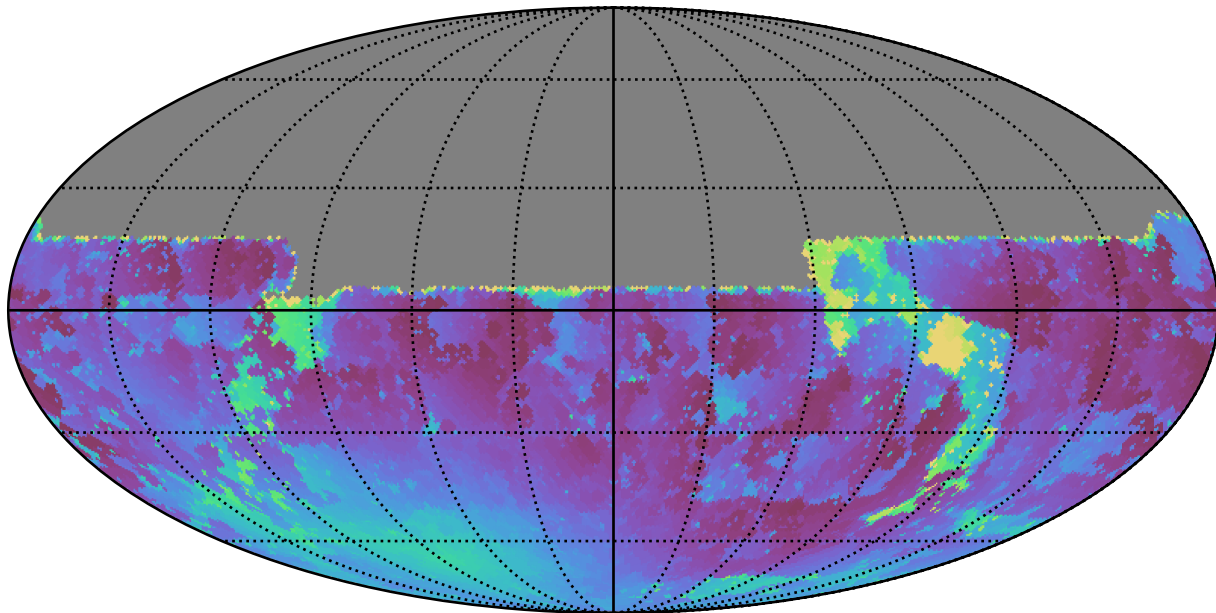
weather_cloudso2v3.4_10yrs All sky u band: Min moonDistance
