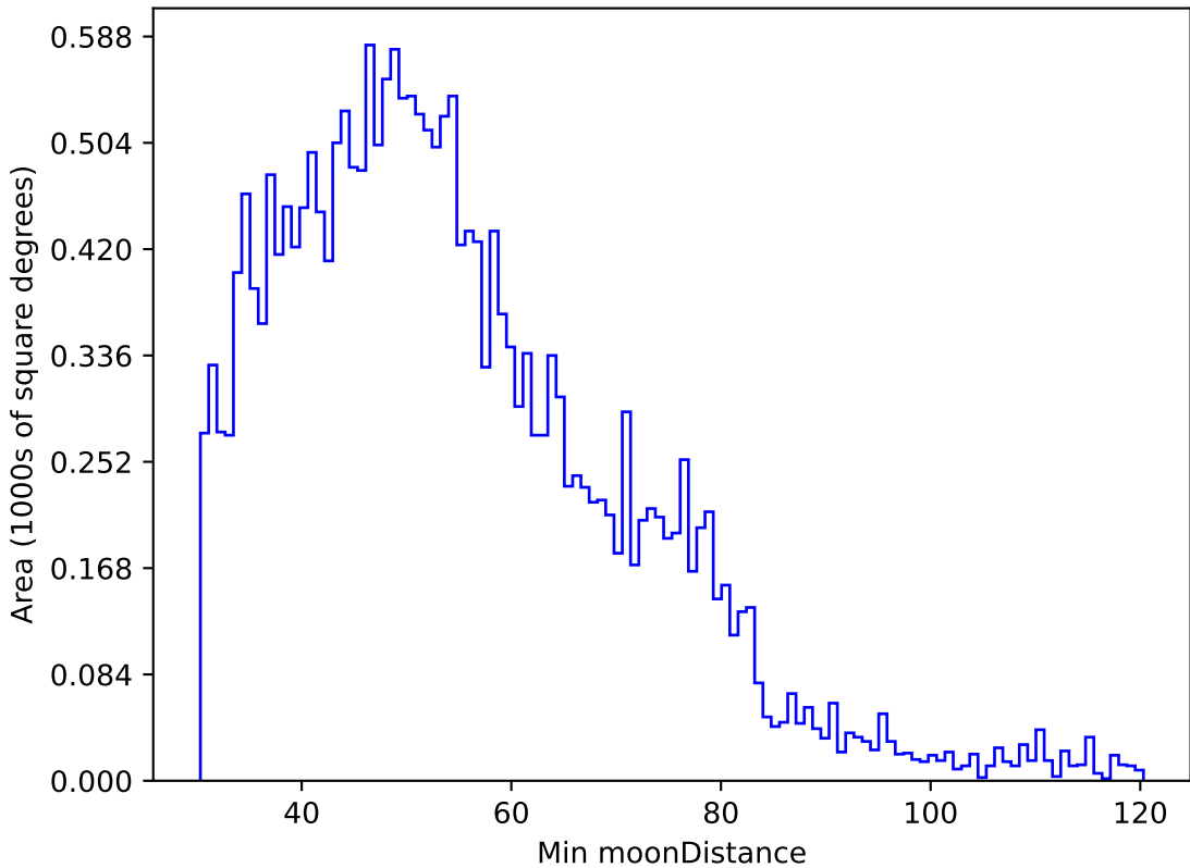
weather_cloudso2v3.4_10yrs All sky u band: Min moonDistance
