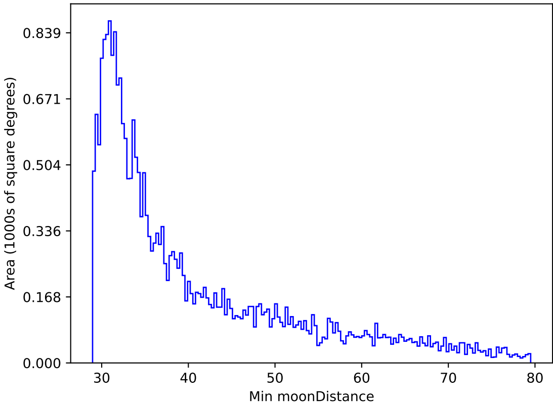
weather_cloudso2v3.4_10yrs All sky r band: Min moonDistance
