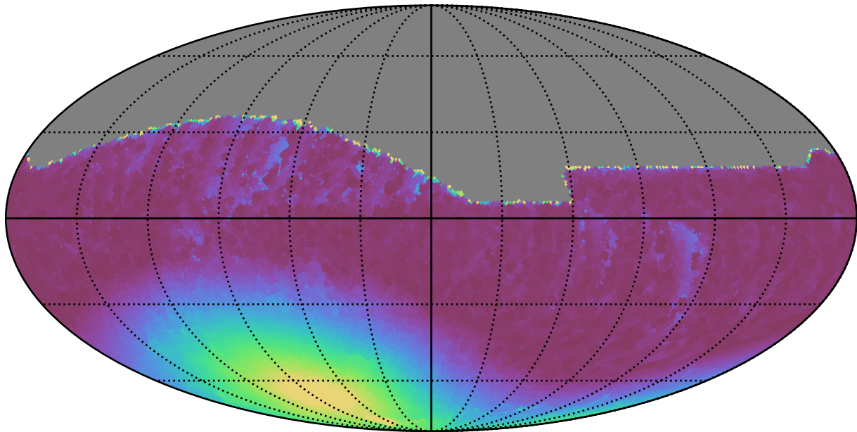
weather_cloudso2v3.4_10yrs All sky i band: Min moonDistance
