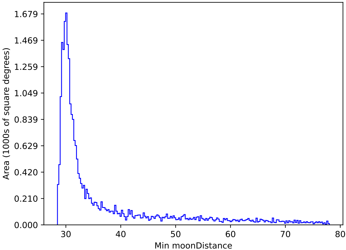
weather_cloudso2v3.4_10yrs All sky i band: Min moonDistance
