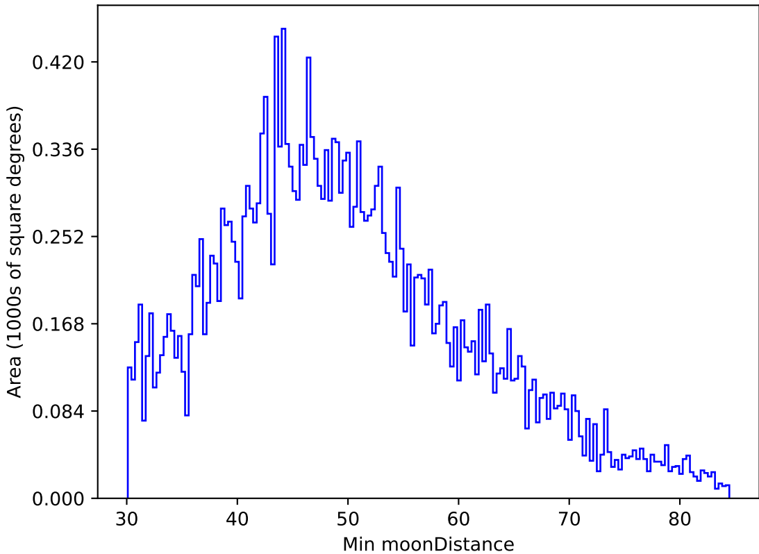
weather_cloudso2v3.4_10yrs All sky g band: Min moonDistance
