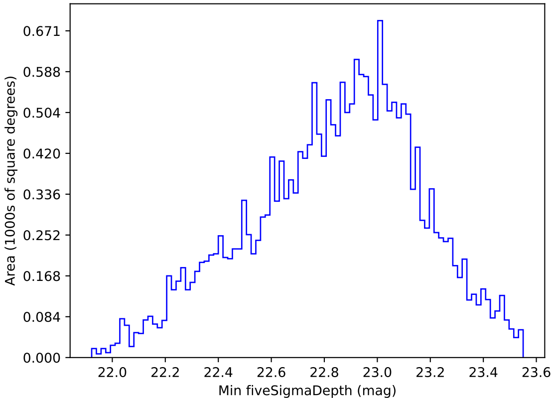
weather_cloudso2v3.4_10yrs Yr 1 u band: Min fiveSigmaDepth
