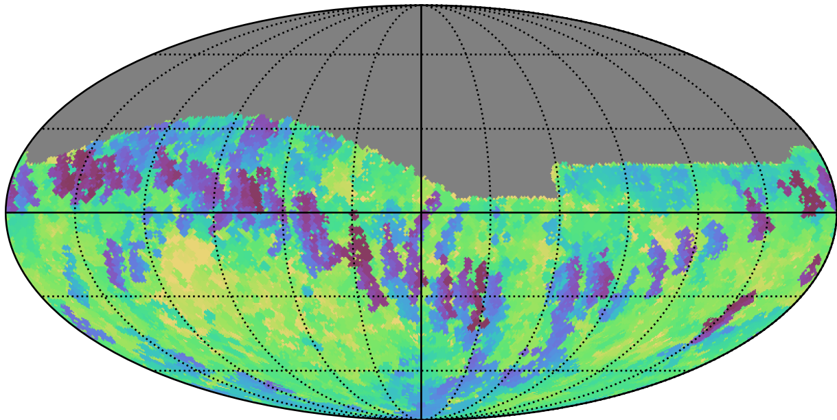
weather_cloudso2v3.4_10yrs Yr 1 i band: Min fiveSigmaDepth
