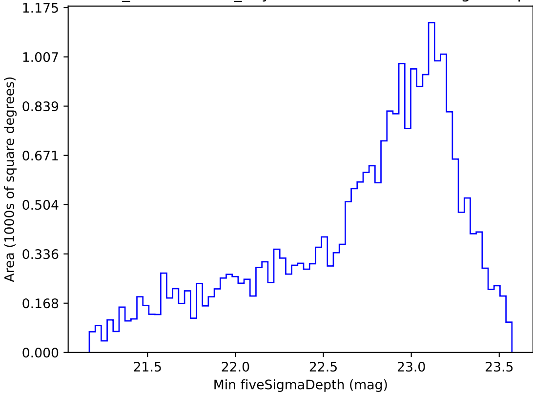
weather_cloudso2v3.4_10yrs Yr 1 i band: Min fiveSigmaDepth
