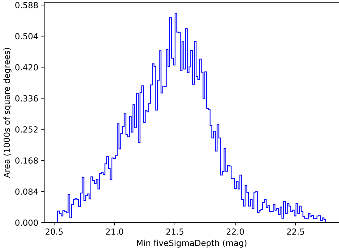
weather_cloudso2v3.4_10yrs Yr 1 all bands: Min fiveSigmaDepth
