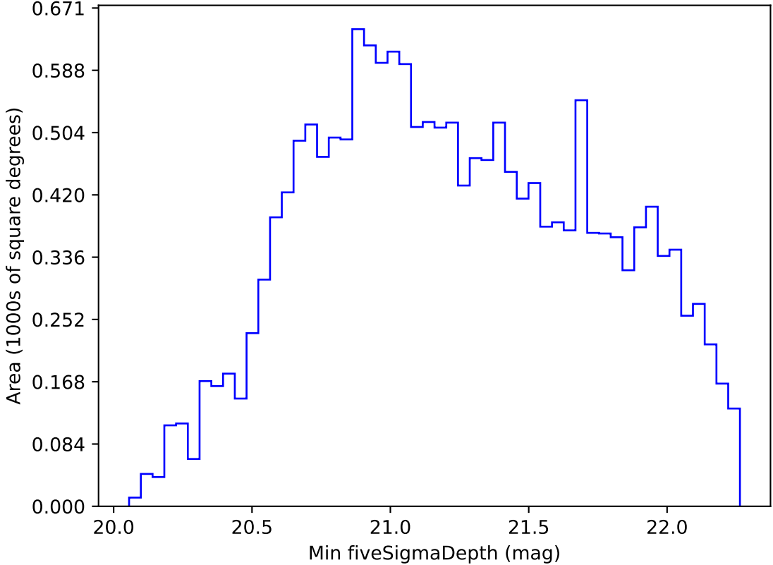
weather_cloudso2v3.4_10yrs WFD z band: Min fiveSigmaDepth
