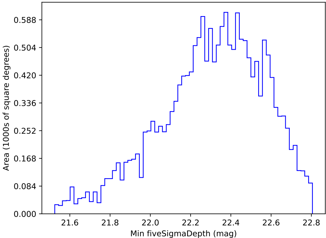
weather_cloudso2v3.4_10yrs WFD u band: Min fiveSigmaDepth
