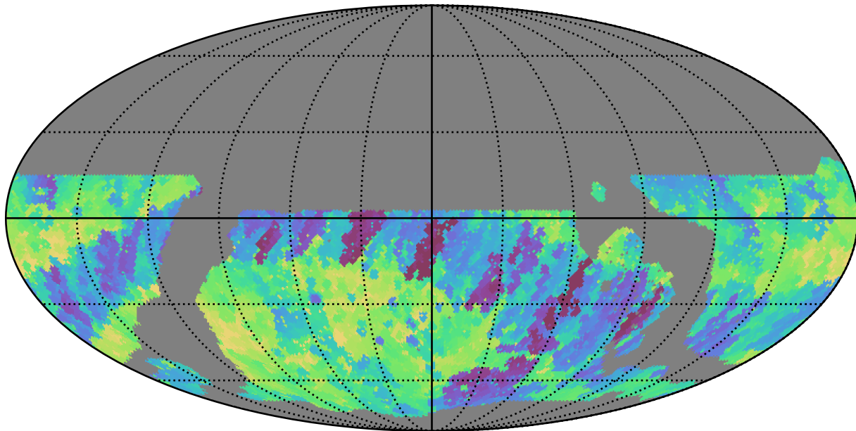
weather_cloudso2v3.4_10yrs WFD r band: Min fiveSigmaDepth
