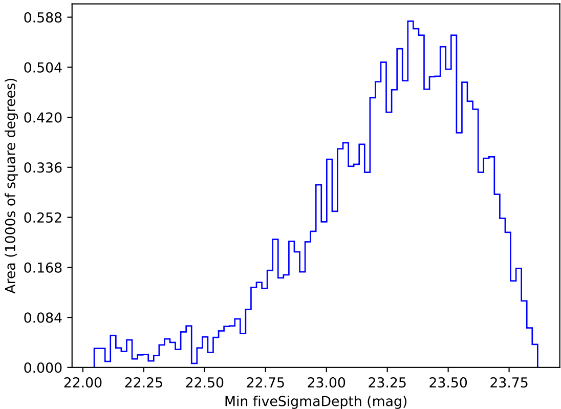
weather_cloudso2v3.4_10yrs WFD g band: Min fiveSigmaDepth
