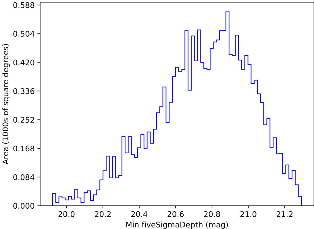
weather_cloudso2v3.4_10yrs WFD all bands: Min fiveSigmaDepth
