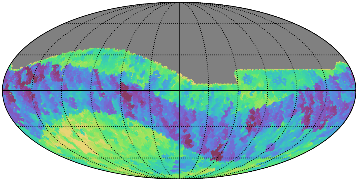
weather_cloudso2v3.4_10yrs All sky z band: Min fiveSigmaDepth
