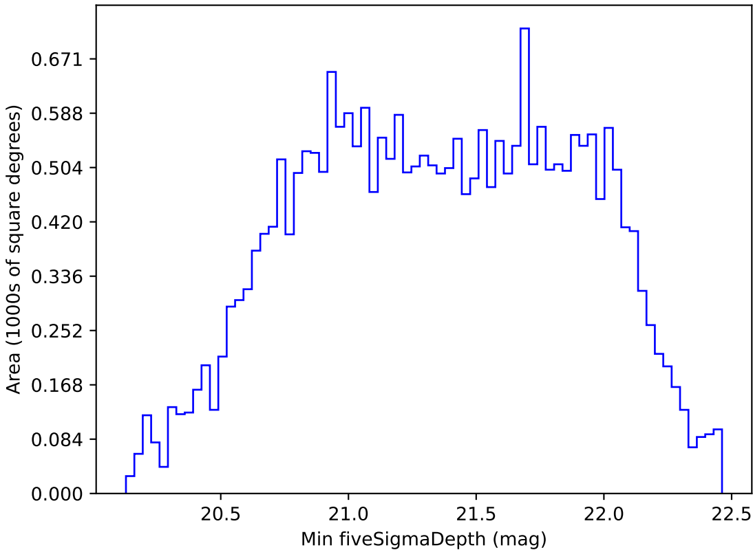
weather_cloudso2v3.4_10yrs All sky z band: Min fiveSigmaDepth
