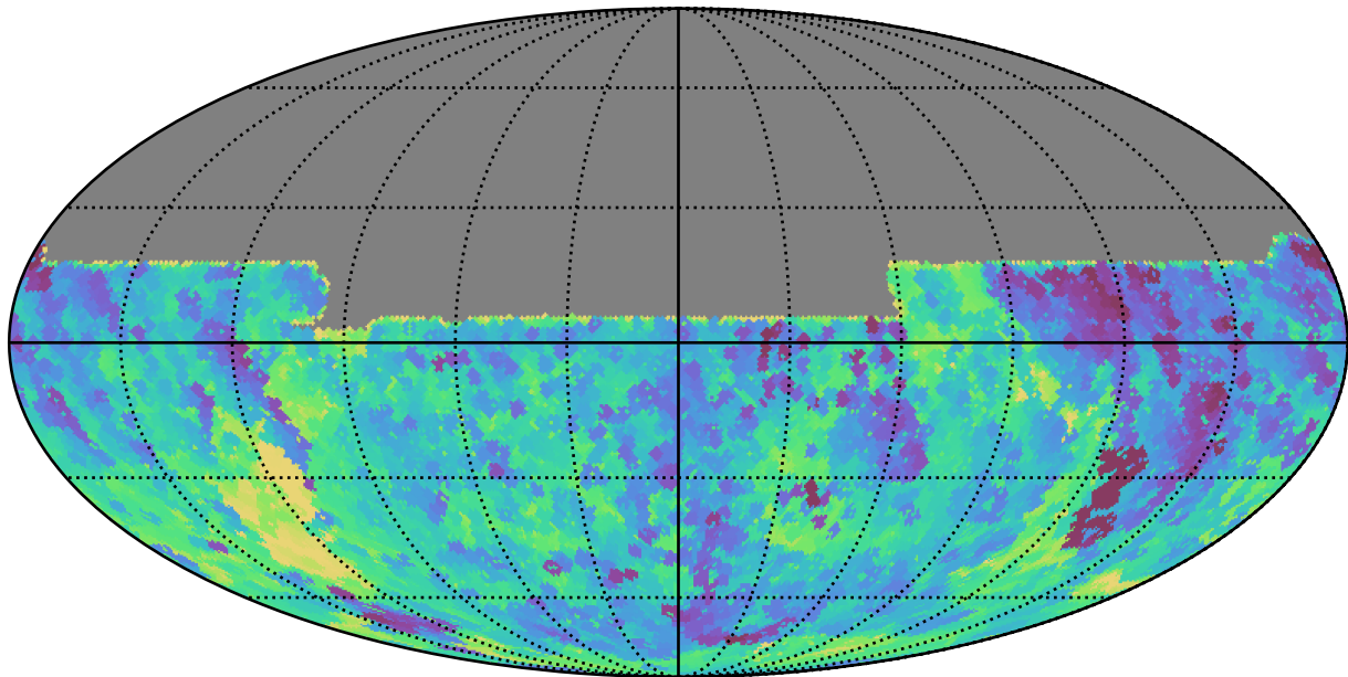
weather_cloudso2v3.4_10yrs All sky y band: Min fiveSigmaDepth
