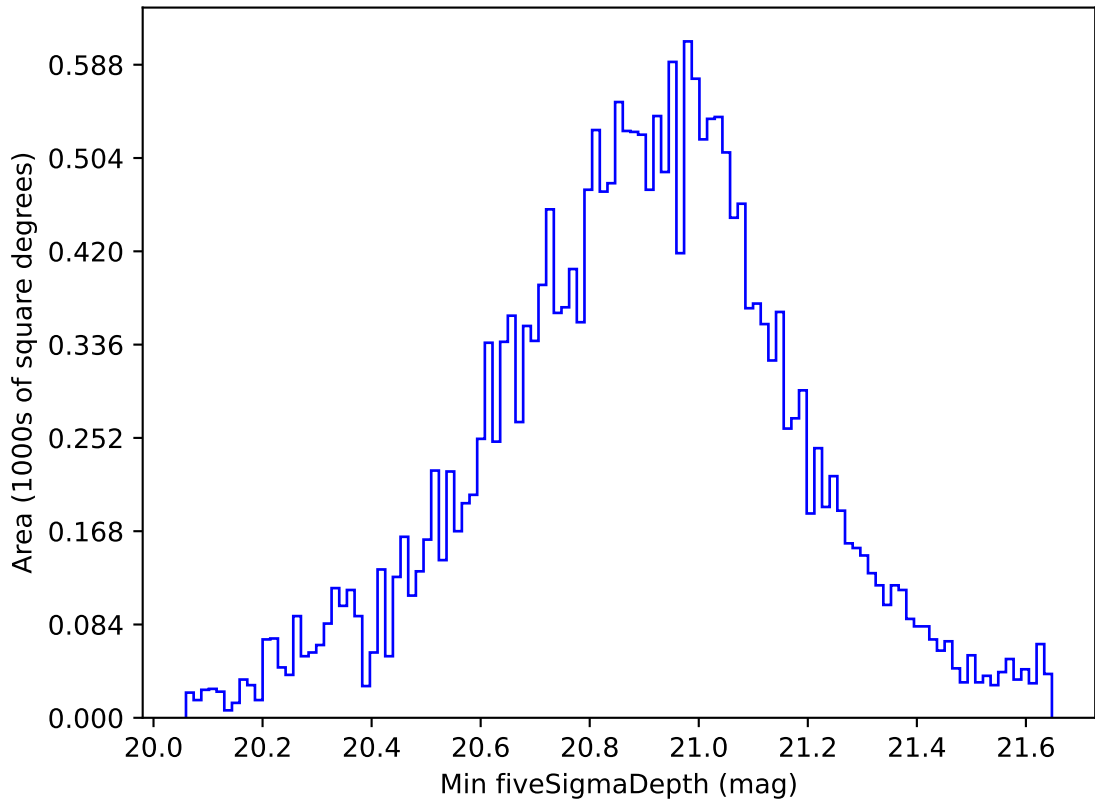
weather_cloudso2v3.4_10yrs All sky y band: Min fiveSigmaDepth
