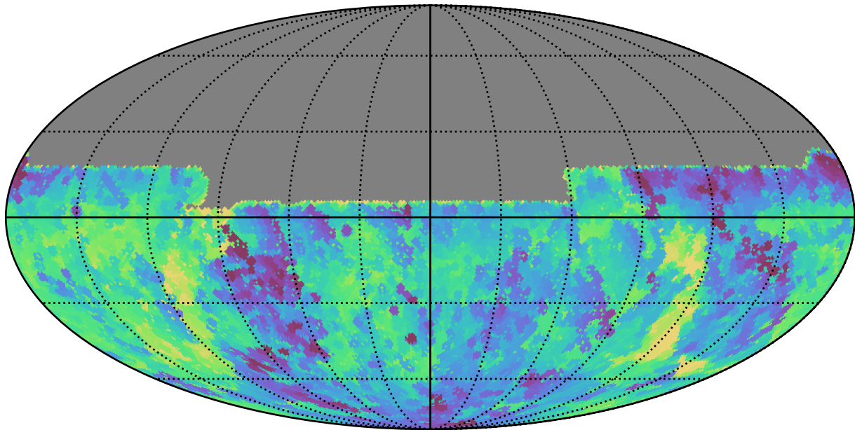
weather_cloudso2v3.4_10yrs All sky u band: Min fiveSigmaDepth
