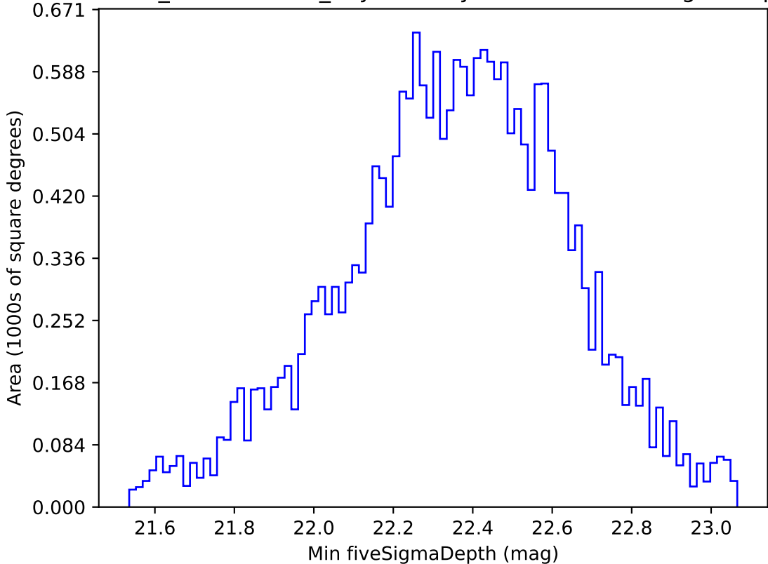
weather_cloudso2v3.4_10yrs All sky u band: Min fiveSigmaDepth
