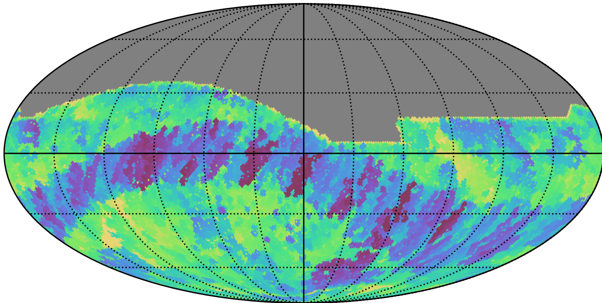
weather_cloudso2v3.4_10yrs All sky r band: Min fiveSigmaDepth
