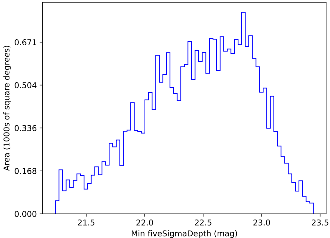
weather_cloudso2v3.4_10yrs All sky r band: Min fiveSigmaDepth
