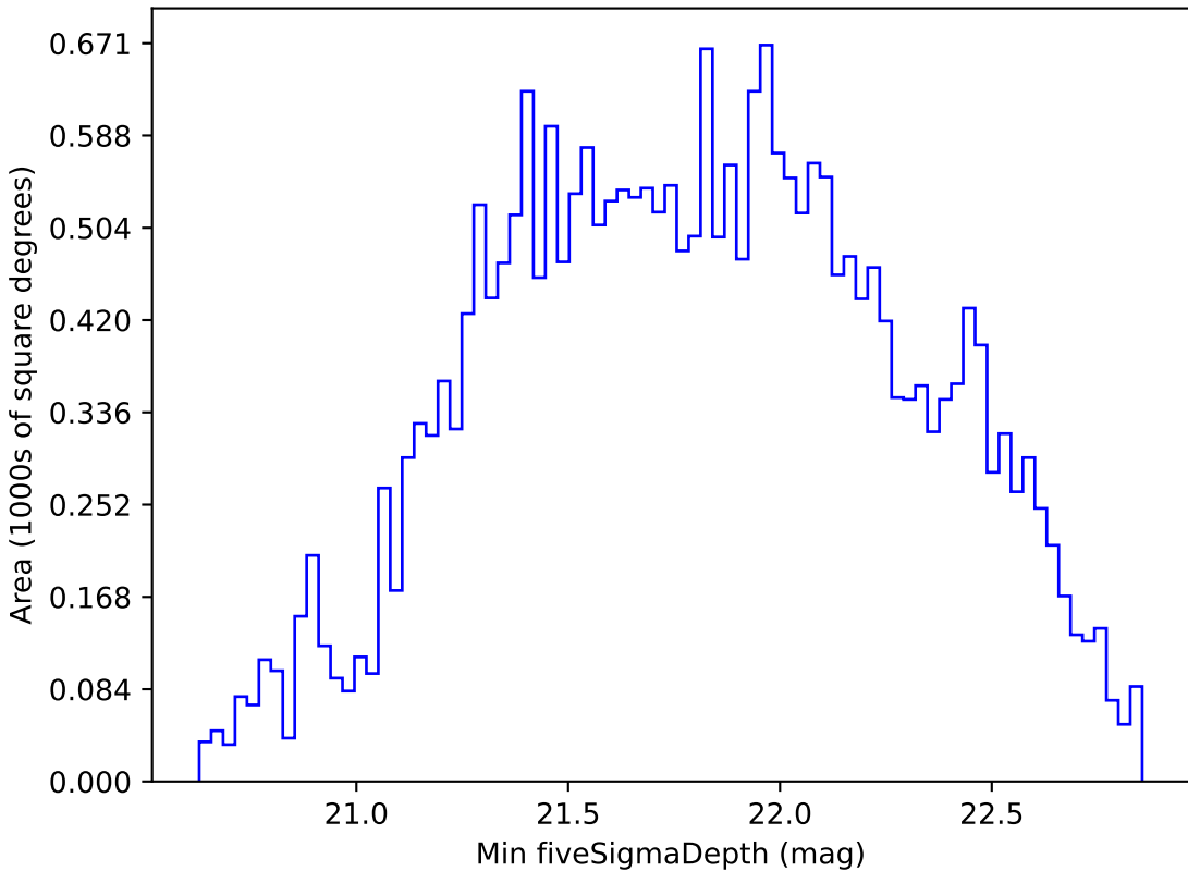
weather_cloudso2v3.4_10yrs All sky i band: Min fiveSigmaDepth
