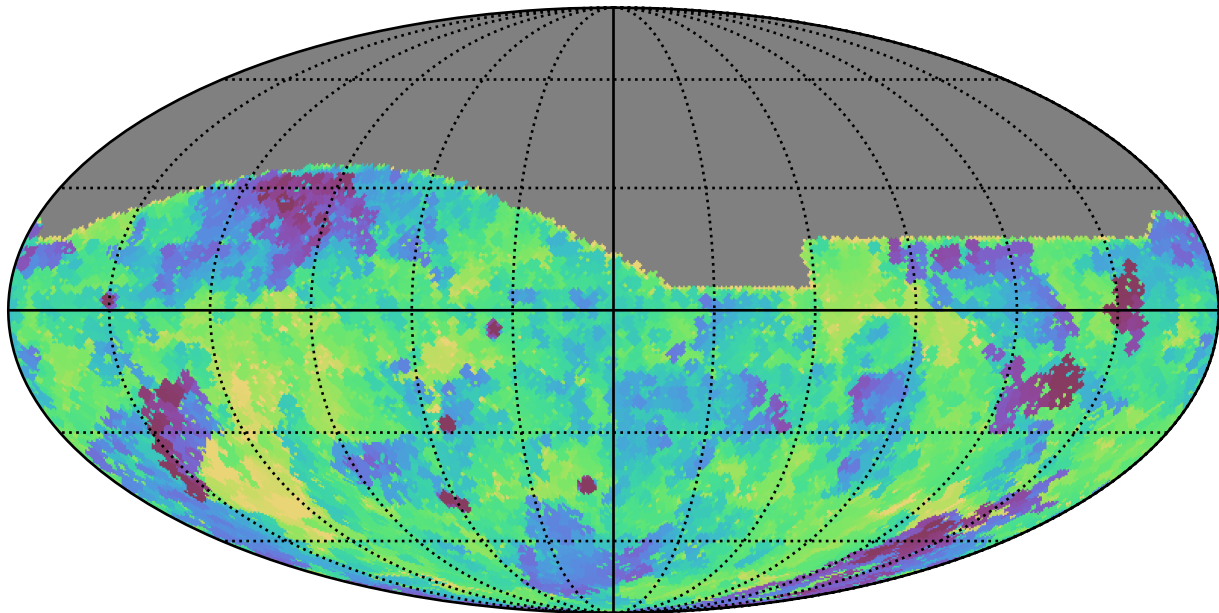
weather_cloudso2v3.4_10yrs All sky g band: Min fiveSigmaDepth
