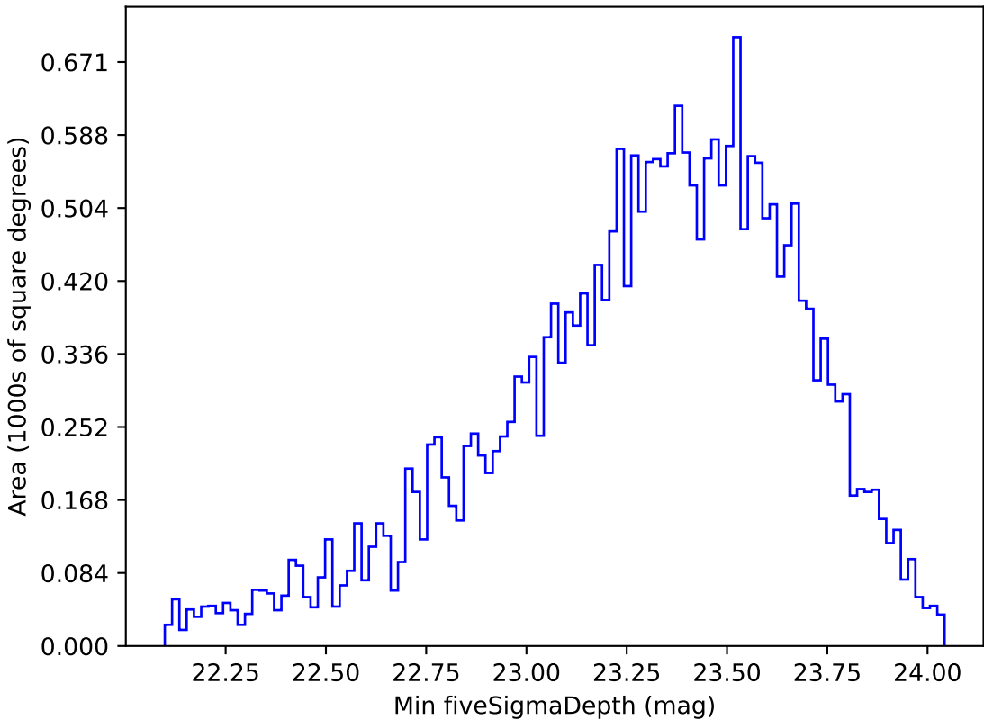
weather_cloudso2v3.4_10yrs All sky g band: Min fiveSigmaDepth
