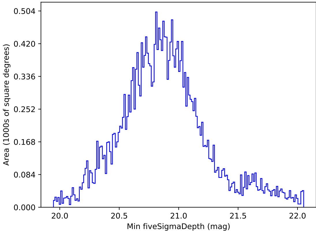
weather_cloudso2v3.4_10yrs All sky all bands: Min fiveSigmaDepth
