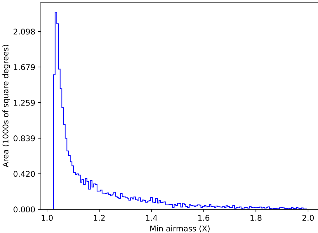
weather_cloudso2v3.4_10yrs Yr 1 z band: Min airmass
