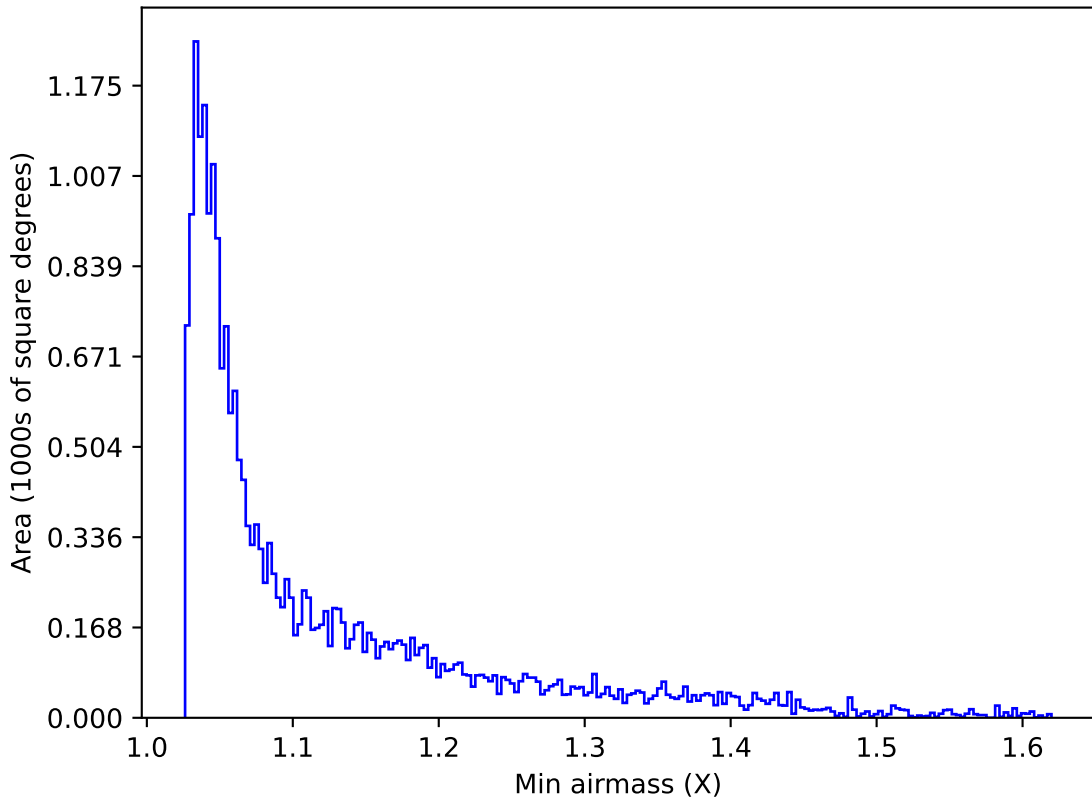
weather_cloudso2v3.4_10yrs Yr 1 y band: Min airmass
