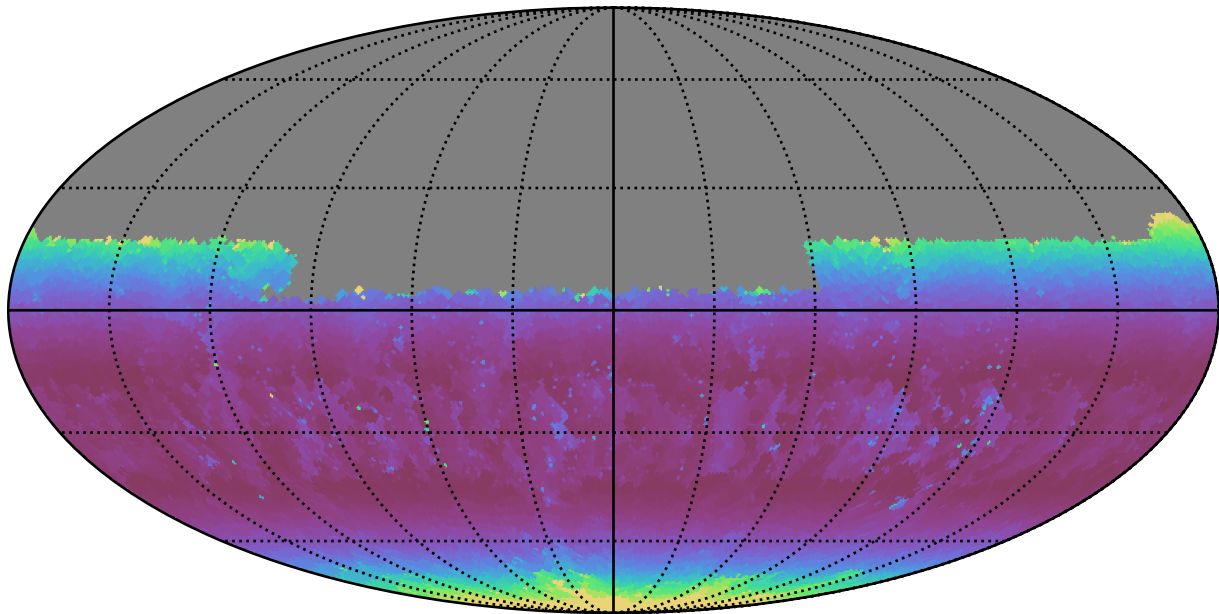
weather_cloudso2v3.4_10yrs Yr 1 u band: Min airmass
