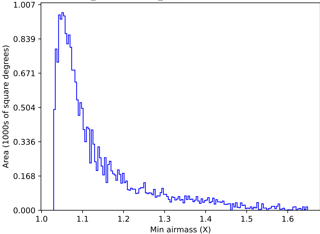
weather_cloudso2v3.4_10yrs Yr 1 u band: Min airmass
