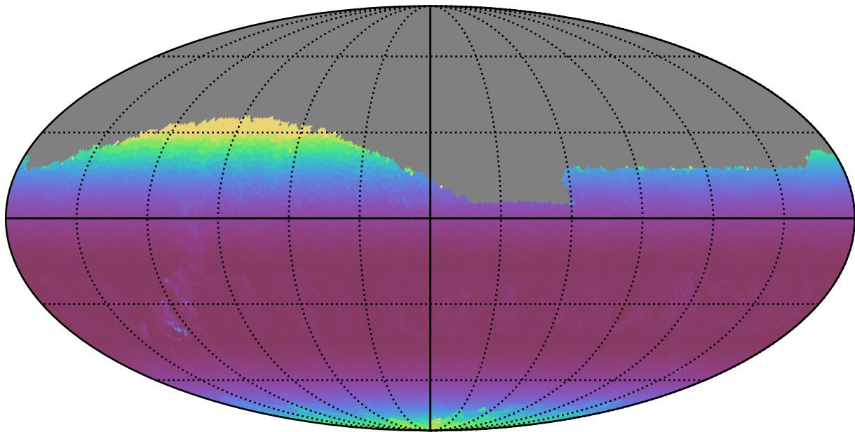
weather_cloudso2v3.4_10yrs Yr 1 r band: Min airmass
