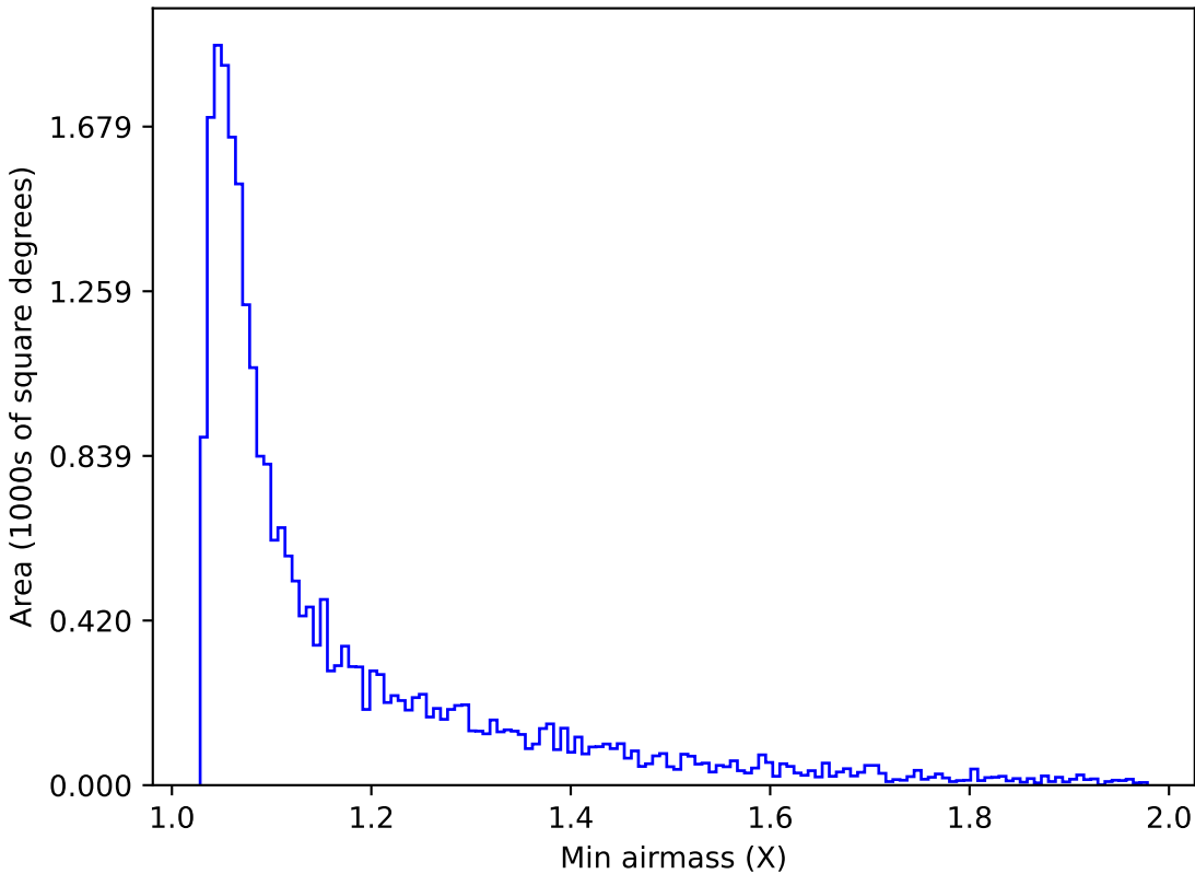
weather_cloudso2v3.4_10yrs Yr 1 g band: Min airmass
