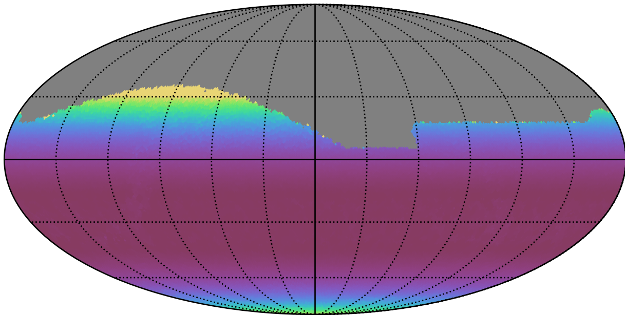
weather_cloudso2v3.4_10yrs Yr 1 all bands: Min airmass
