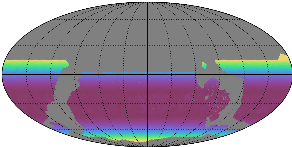
weather_cloudso2v3.4_10yrs WFD z band: Min airmass
