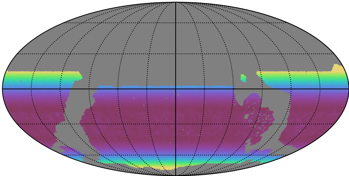
weather_cloudso2v3.4_10yrs WFD y band: Min airmass
