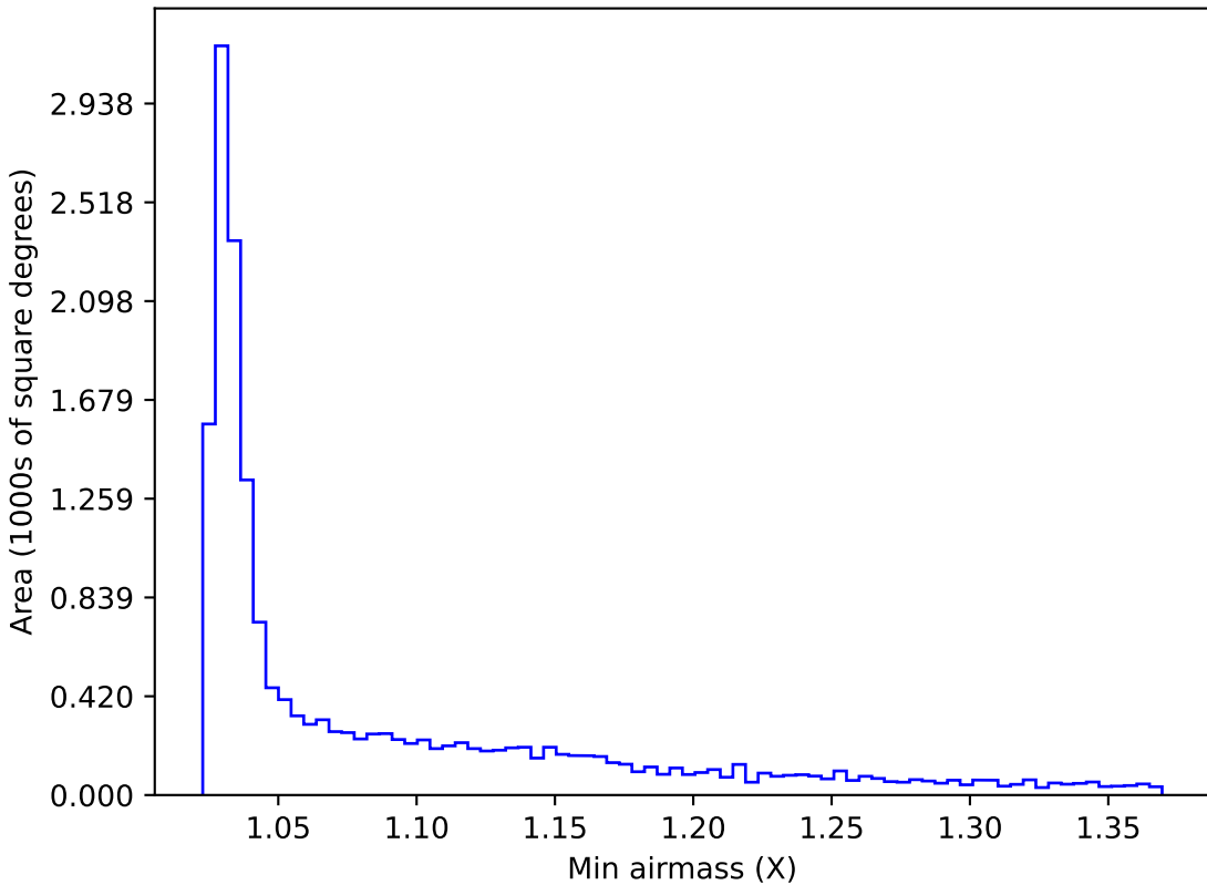
weather_cloudso2v3.4_10yrs WFD y band: Min airmass
