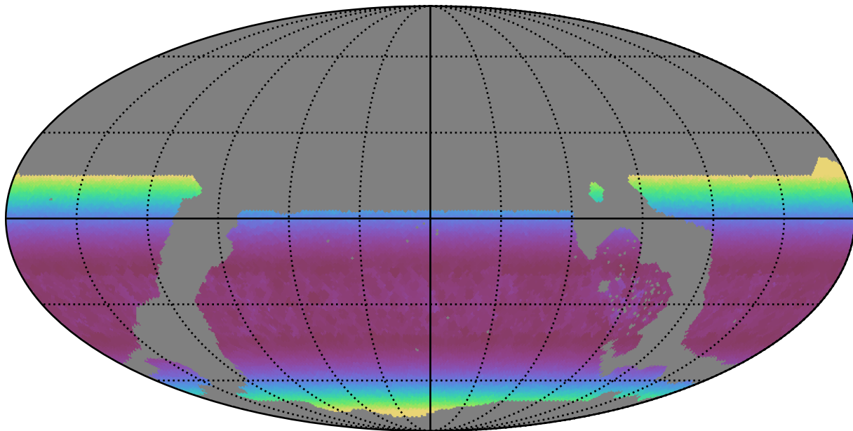
weather_cloudso2v3.4_10yrs WFD u band: Min airmass
