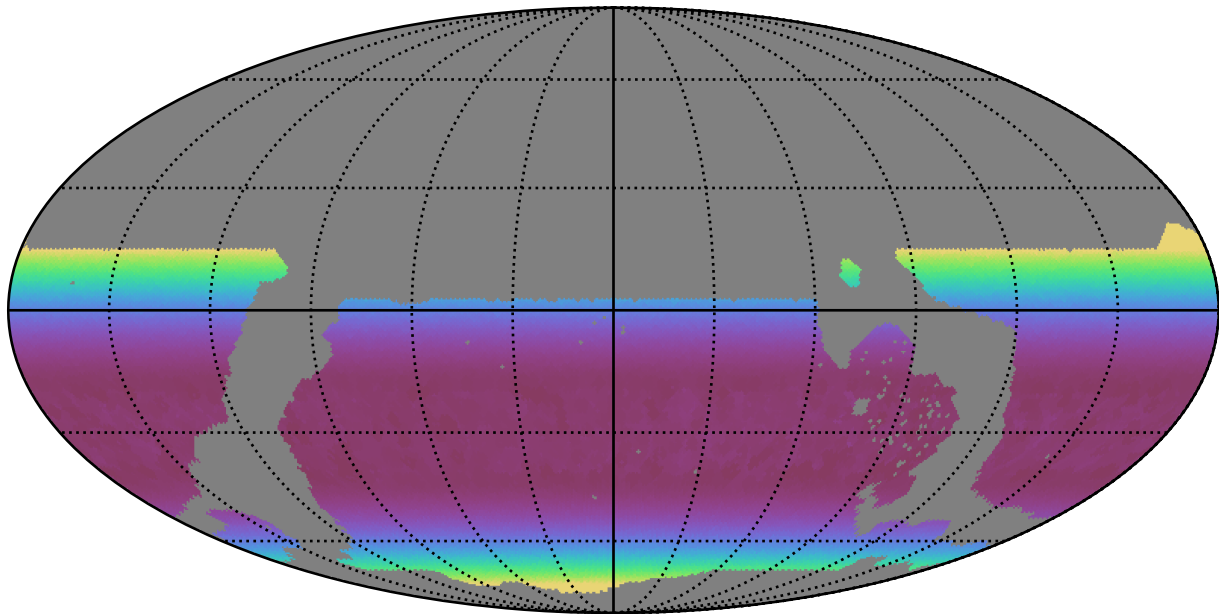
weather_cloudso2v3.4_10yrs WFD i band: Min airmass
