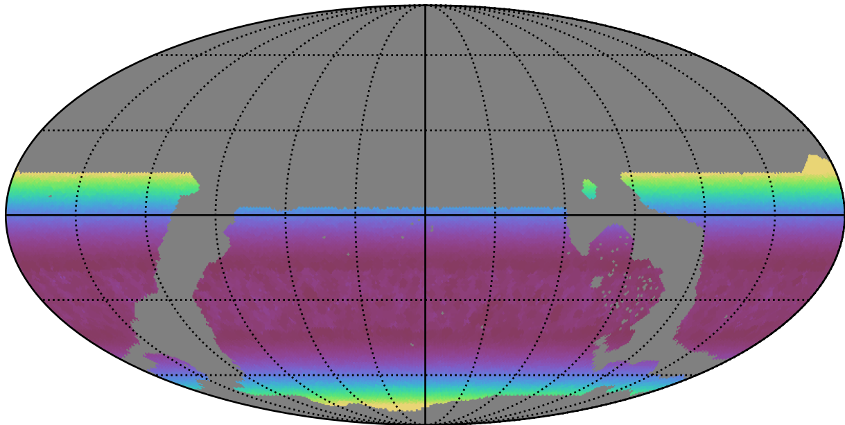
weather_cloudso2v3.4_10yrs WFD g band: Min airmass
